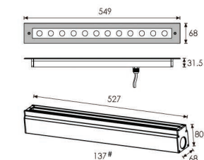
Mounting Sleeve137#
