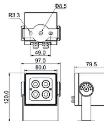
Product Dimension
