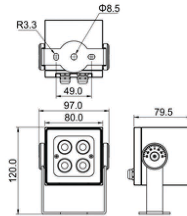
Product Dimension
