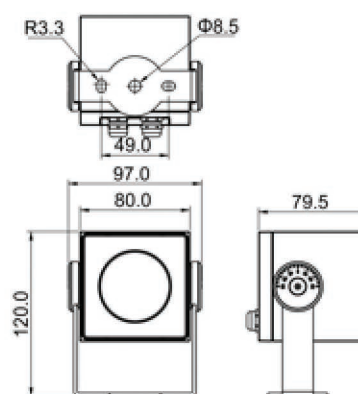
Product Dimension
