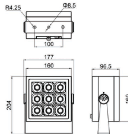
Product Dimension
