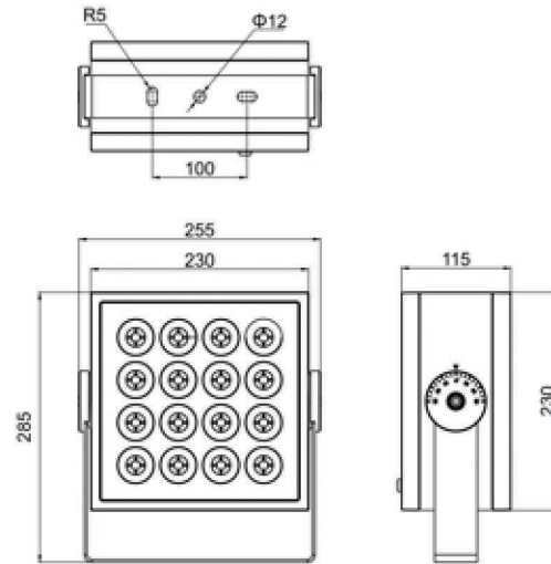
Product Dimension
