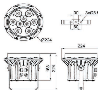
Product Dimension
