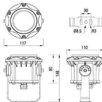
Product Dimension
