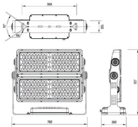
Product Dimension
