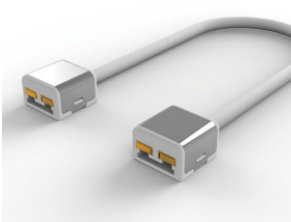
IP20 Jumper connector 10A (tape-wire-tape)
