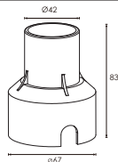
Mounting sleeve 033#
